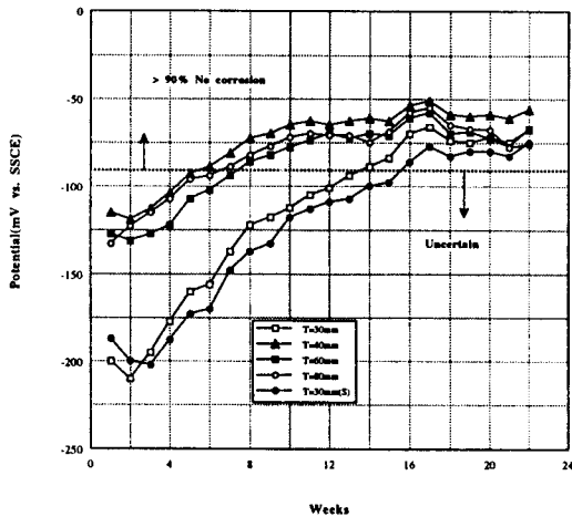
Fig.5 Potential variation of rebar at different cover thickness(LFC)
