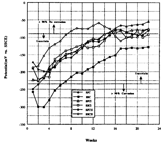
Fig.4 Potential variation of SFC and SSC series specimens with or without inhibitor
