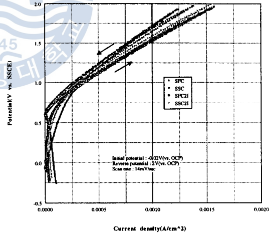
Fig.8 Linear plots for Fig.7
