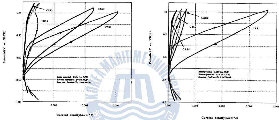
Fig.9 Linear cyclic polarization curves for mortar specimens made by 4.3% inhibitor (7 years) Fig.10 Linear cyclic polarization curves for mortar specimens made by 8.6% inhibitor(7 years)
