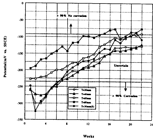
Fig.6 Potential variation of rebar at different cover thickness(SSC)
