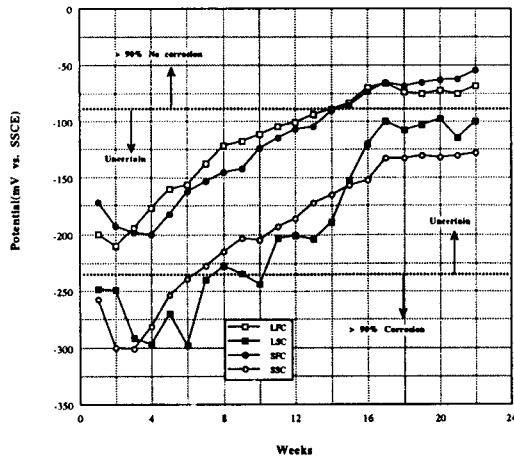
Fig.3 Potential variation of four specimens with time(cover thickness 30mm)
