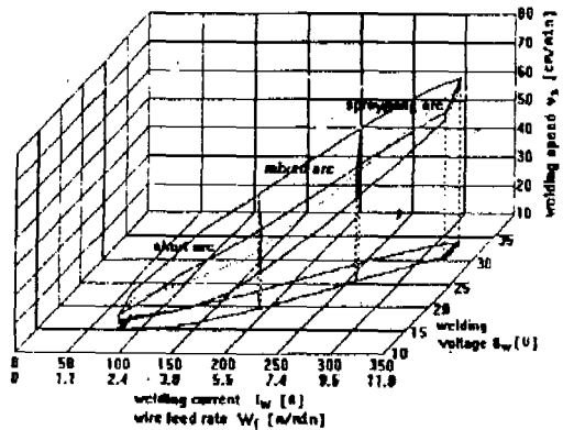
Fig. 1 Three dimensional representation of usable area of welding parameters
