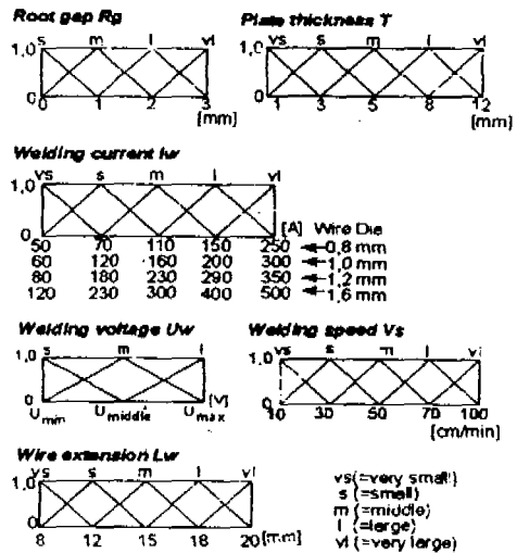
Fig. 3 Evaluation of welding parameters by fuzzy sets
