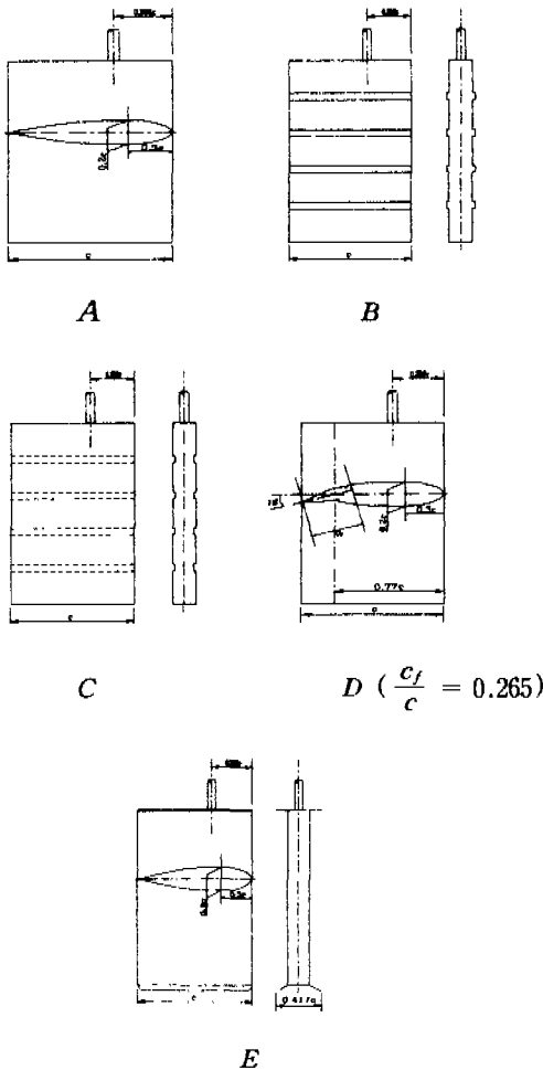
Fig. 5 Model rudders
