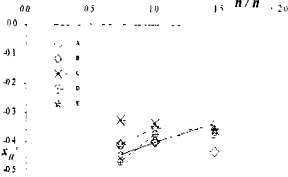
Fig. 13 Effect of propeller load on hull-rudder interaction factor x_{HH}'
