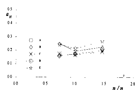
Fig. 12 Effect of propeller load on hull-rudder interaction factor a_H
