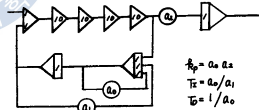
Fig. (8) Simulation program of the PID controller
