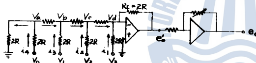
Fig. (15) 2R, R Ladder network
