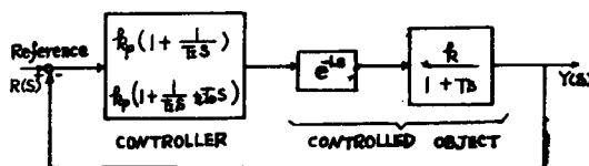
Fig. (1) The block diagram of the feed back control system
