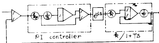
Fig. (19) The connection diagram of the analog simulation system when the PI controller is used
