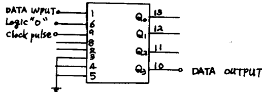
Fig. (14) Pin connection diagram of the Shift register
