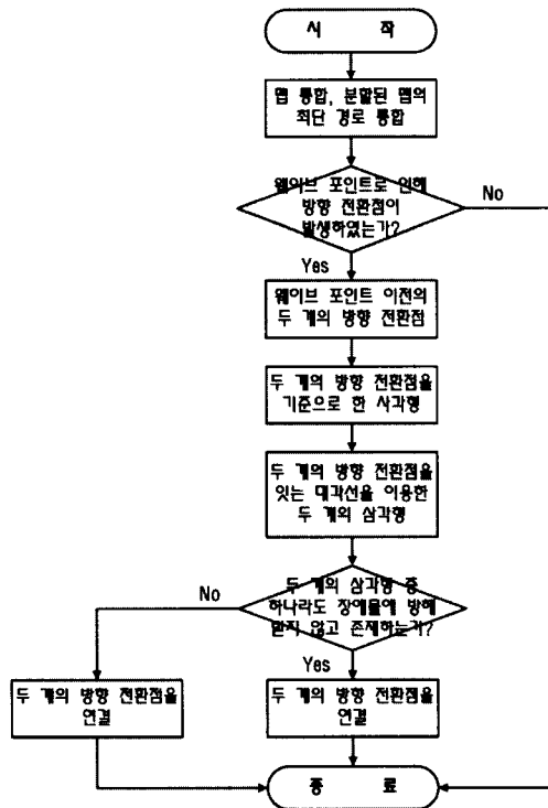
Fig. 8 Flowchart of the path amendment algorithm
