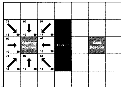
Fig. 3 Calculation of f, g and h cost
