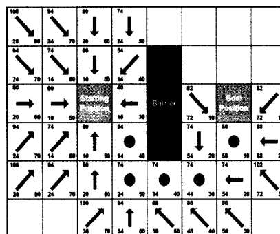
Fig. 5 Example of the shortest course creation
