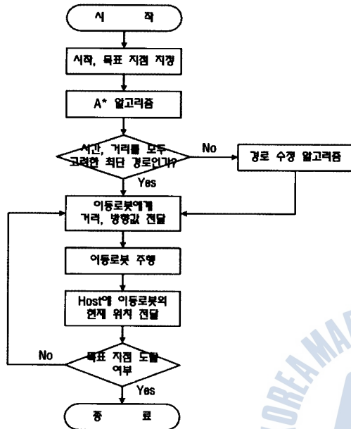
Fig. 11 Flowchart of the traveling algorithm
