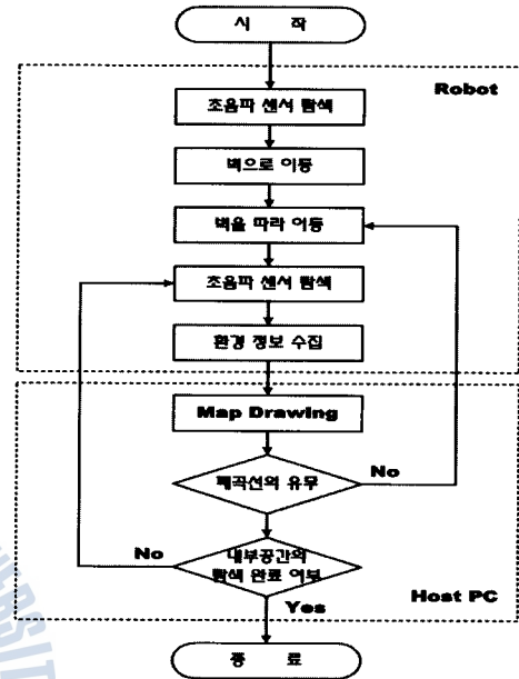
Fig. 1 Flowchart of the map building algorithm
