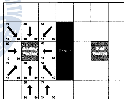
Fig. 4 Repetitive accomplishment of the A* algorithm
