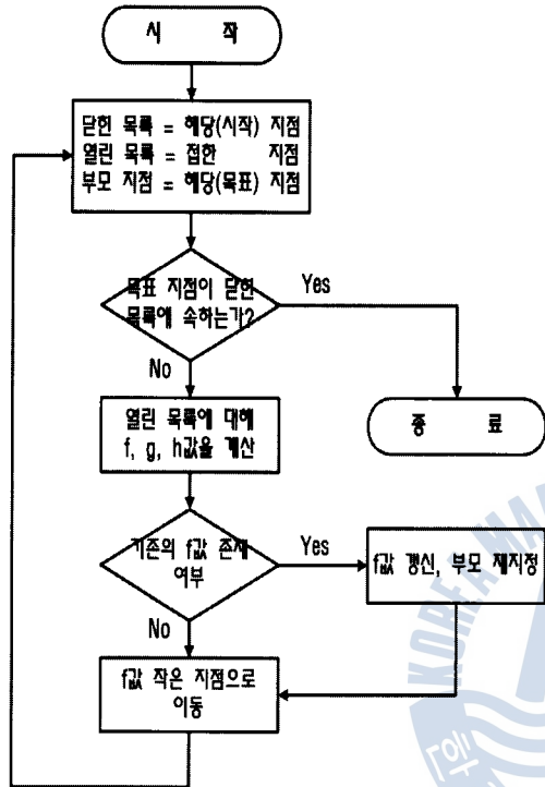
Fig. 6 Flowchart of the A* algorithm
