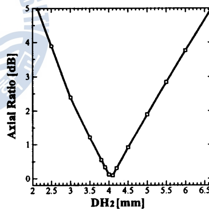
Fig. 12 Axial ratio for the variation of DH2
