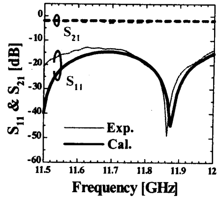
Fig. 7 Comparison between calculation and experiment
