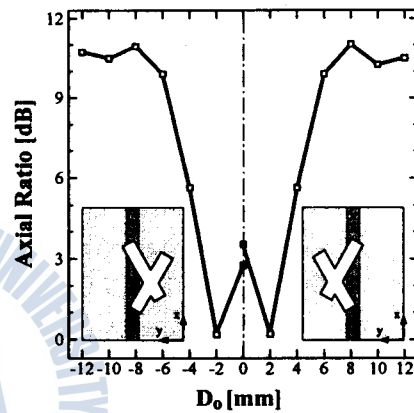
(a) Axial ratio
