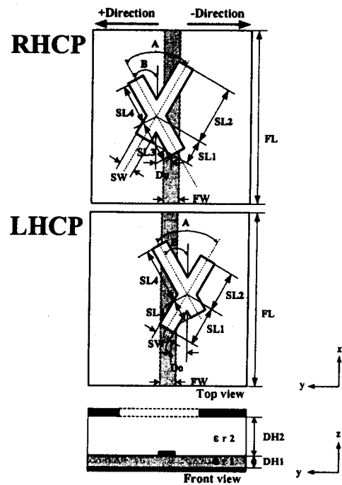
Fig. 1 Structure of 1-element cross slot antenna
