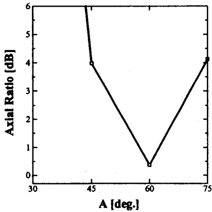
Fig. 3 Axial ratio for the variation of A
