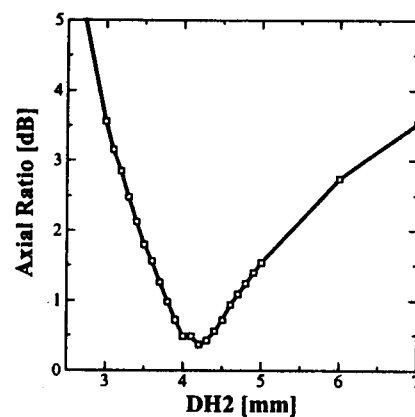
Fig. 2 Axial ratio for the variation of DH2
