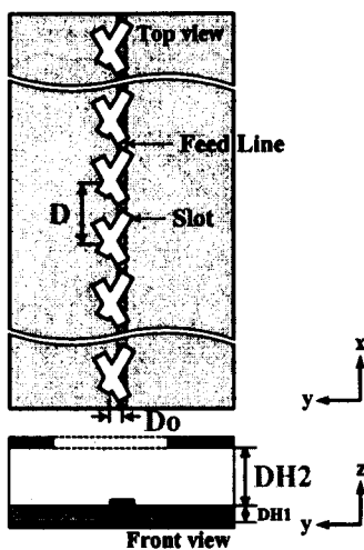
Fig. 10 Structure of 15-element cross slot array antenna
