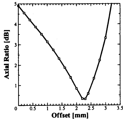
Fig. 11 Axial ratio for the variation of D0
