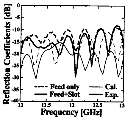
Fig. 15 Comparison between calculation and experiment
