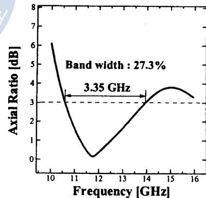
Fig. 8 Axial ratio for the variation of frequency
