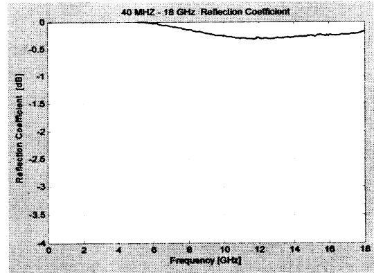
(b) Reflection Coefficient from Pure Silicone Rubber with 5 mm in Thickness..
