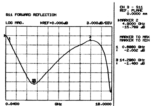
(d) Electromagnetic absorber's reflection coefficient that thickness is 4 mm
