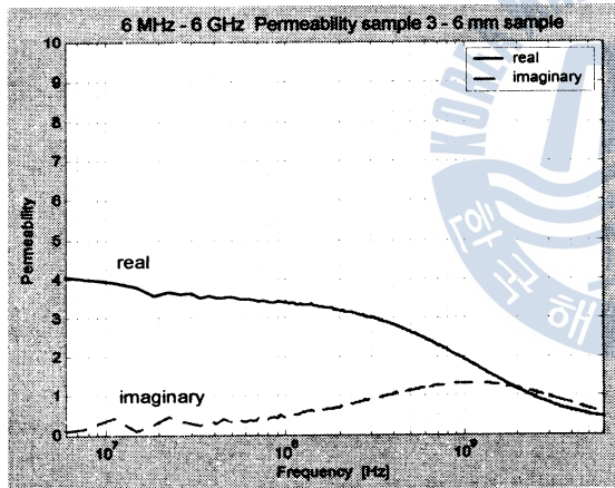
(c) Complex permeability of MnZn ferrite absorber mixed with natural lacquer.
