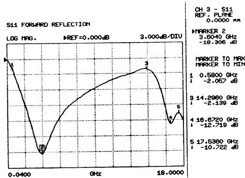
(e) Reflection from Electromagnetic absorber coefficient with the thickness of 5 mm
