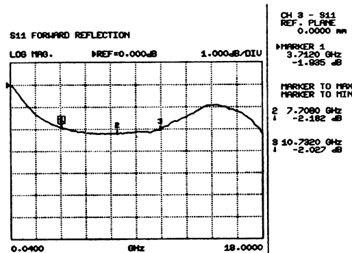
(a) Electromagnetic absorber's reflection coefficient that thickness is 1 mm
