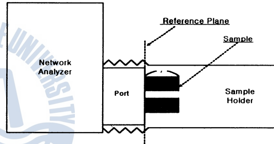
Fig. 1 Reflection coefficient measurement system of sample.
