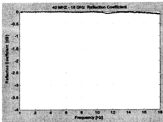
(a) Reflection coefficient from Pure CPE with 5mm in Thickness
