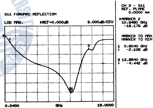
(c) Electromagnetic absorber's reflection coefficient that thickness is 3 mm
