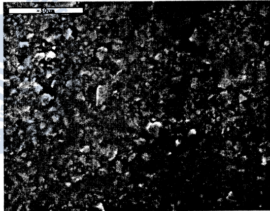
(b) MnZn ferrite mixed with silicone rubber.
