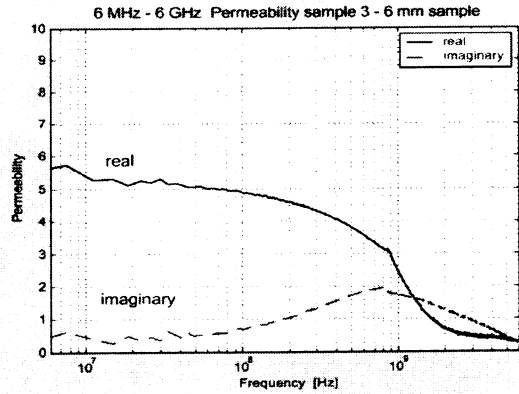
(b) Complex permeability of MnZn ferrite absorber mixed with silicone rubber.
