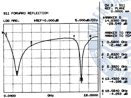
(f) Reflection from Electromagnetic absorber coefficient with the thickness of 6 mm
