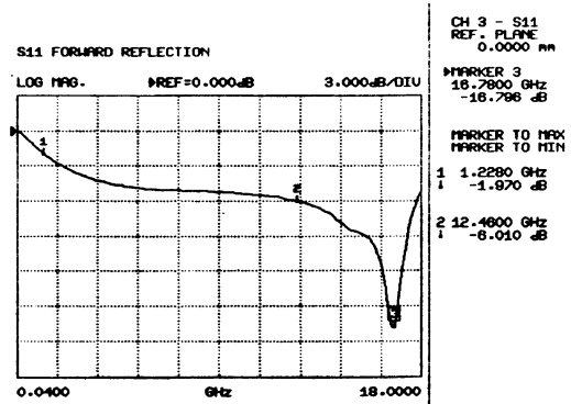
(b) Electromagnetic absorber's reflection coefficient that thickness is 2 mm
