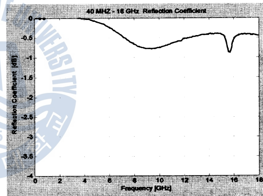
(c) Reflection coefficient from Pure Natural Lacquer with 5 mm. in Thickness.
