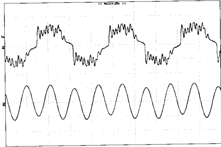
Upper : Total leakage current [500 μA/div, 5ms/div] Lower : Third leakage current [100 μA/div, 5ms/div]
