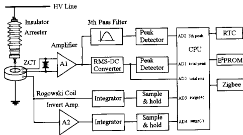
Fig. 1 Configuration of the ubiquitous sensor
