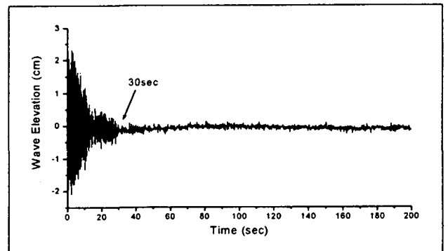
Fig. 4 Time history of wave elevation with wave absorber
