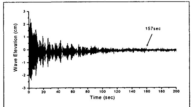
Fig. 3 Time history of wave elevation W/O wave absorber
