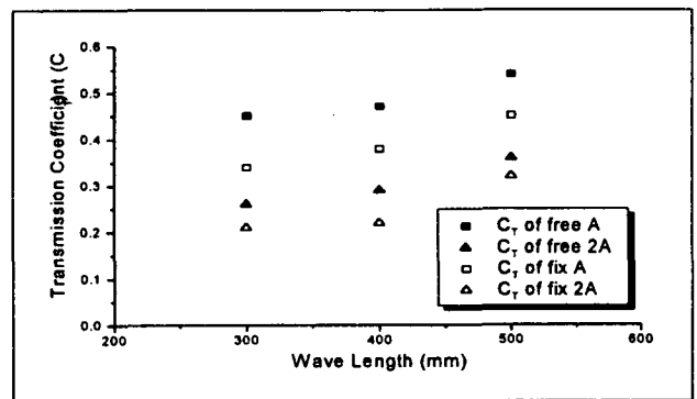
Fig. 8 C_T vs Wave Length
