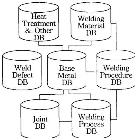
Fig. 1 Database Components and Their Relationships
