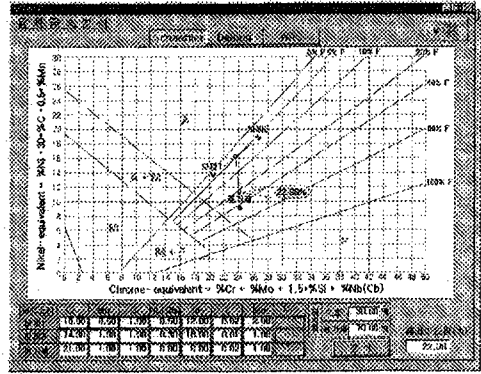
Fig. 9 Calculation of ferrite content
