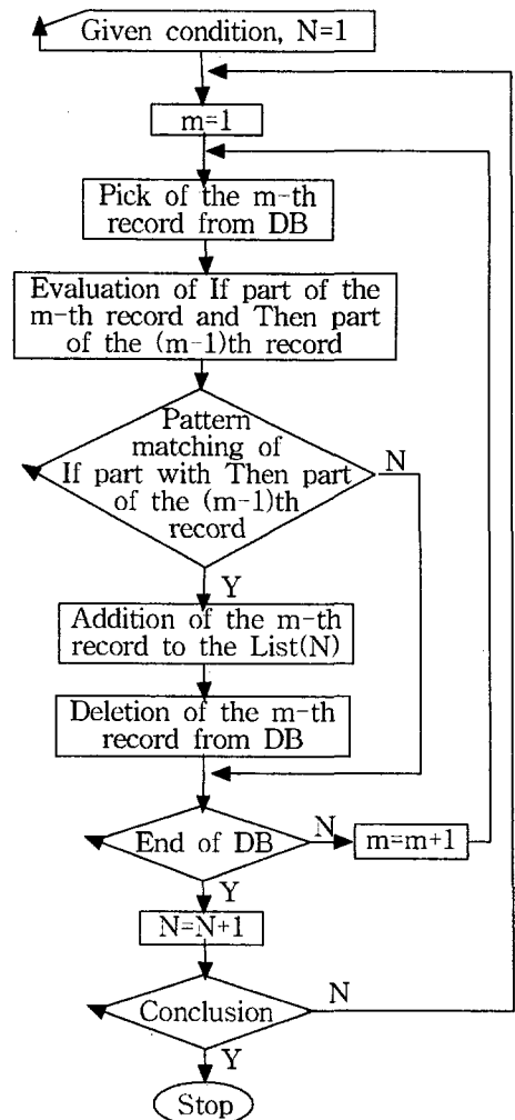
Fig. 3 Inference algorithm using DB
