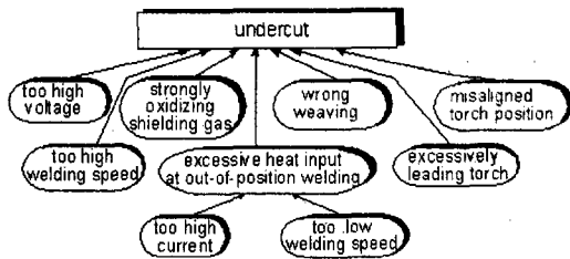
Fig. 7 Causal model of undercut
