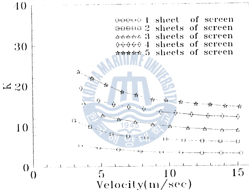
Fig. 4 Characteristics of screen
