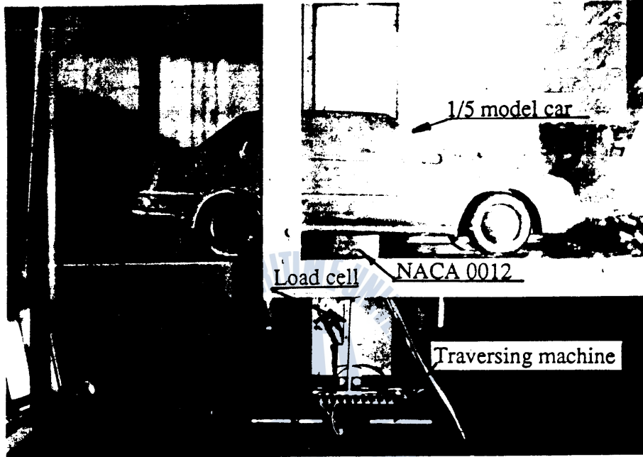
(a) 1/5 model car with balance and supporter
