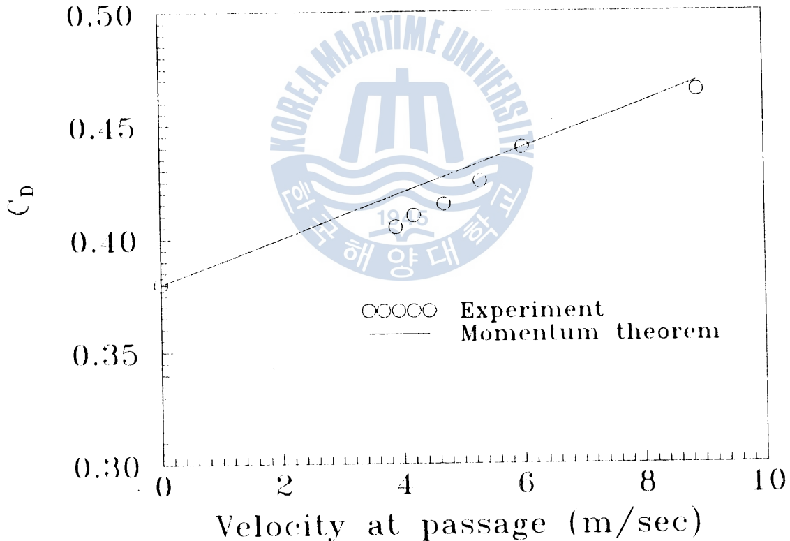
Fig. 7 Comparison of C_D with momentum theorem
