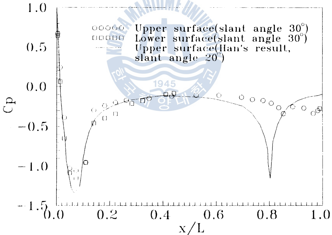
Fig. 6 Comparison of pressure coefficient of upper and lower surface
