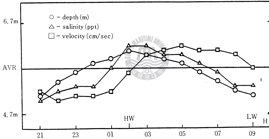
Figure 11. Time variation of depth, velocity & salinity at A(1985. 4, 27)
