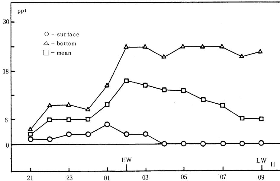
Figure 7. Time variation of salinity at A(1985. 4, 27)
