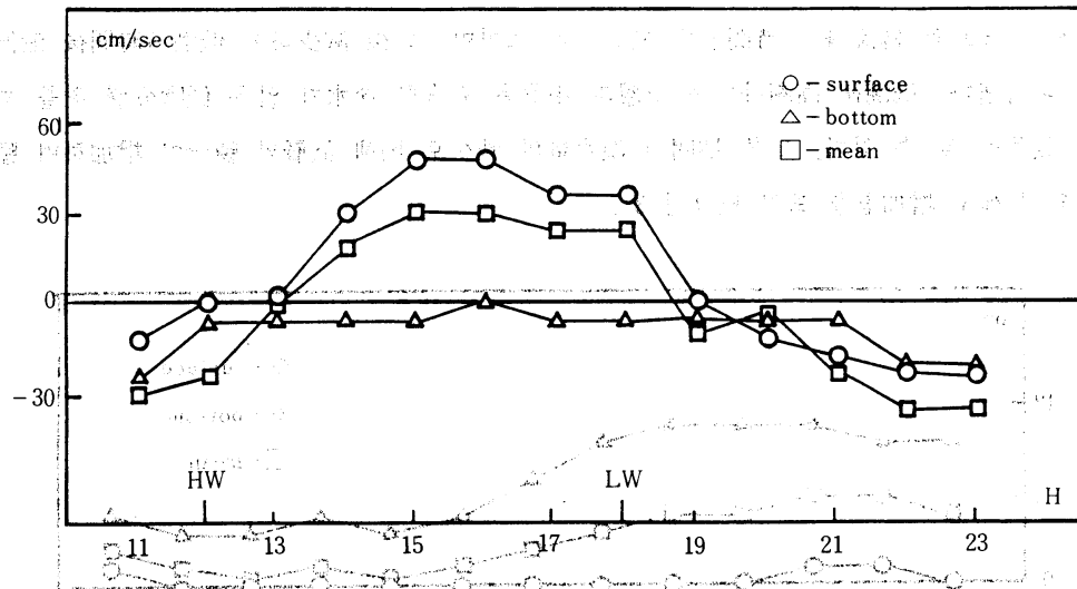
Figure 4. Time variation of velocity at N(1985. 4, 25)
