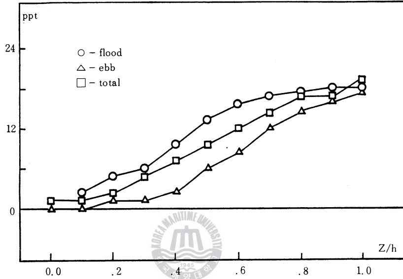
Figure 8. Salinity profile at A(1985. 4, 27)
