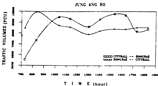
Fig. 4.1 Roadway Traffic Volume Collection @ hhu
