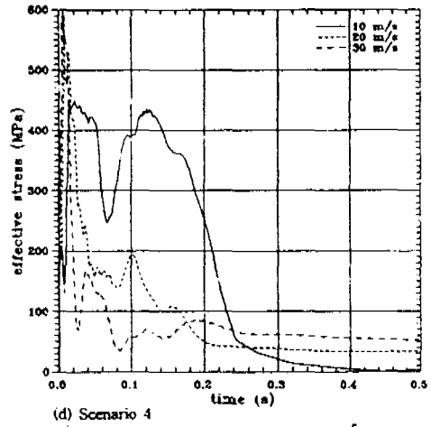
FIGURE 3.2 Time history of effective stress at a point of impact of pipe
