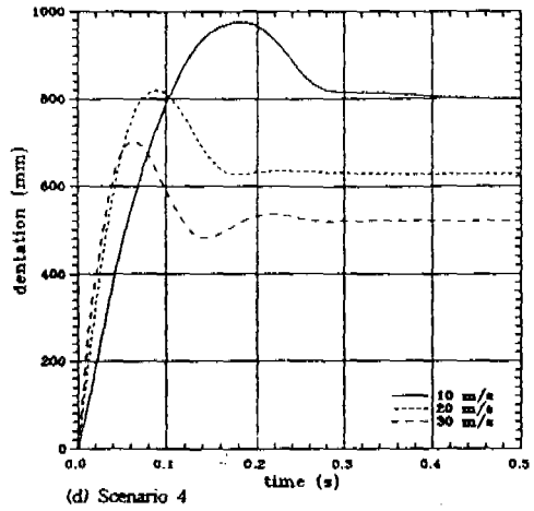
FIGURE 3.3 Time history of depth of dent at a midsection of pipe
