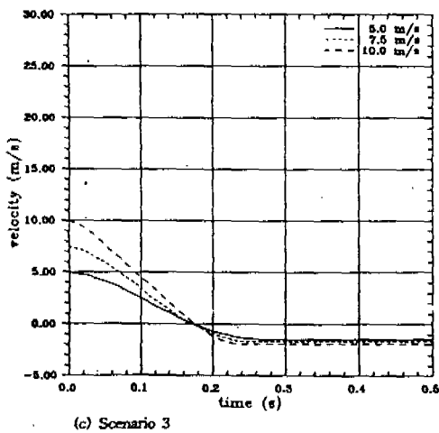
FIGURE 3.4 Time history of velocity of struck pipe
