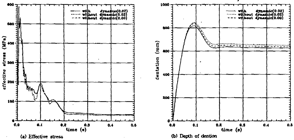
FIGURE 3.6 Effect of strain rate-dependent plasticity
