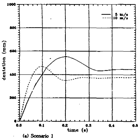
FIGURE 3.3 Time history of depth of dent at a midsection of pipe (continue)
