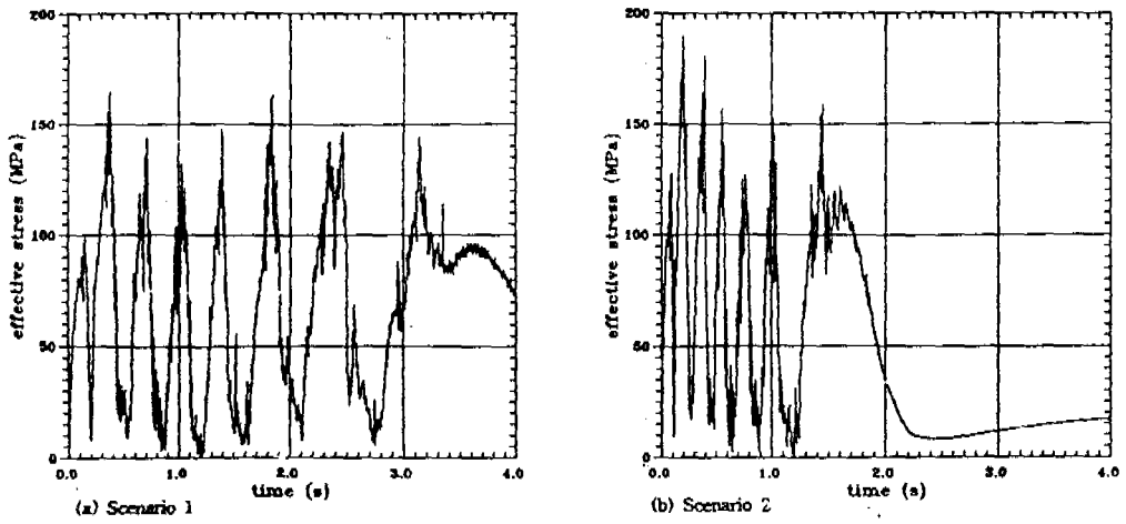
FIGURE 4.3 Time history of effective stress at a point of impact of pipe
