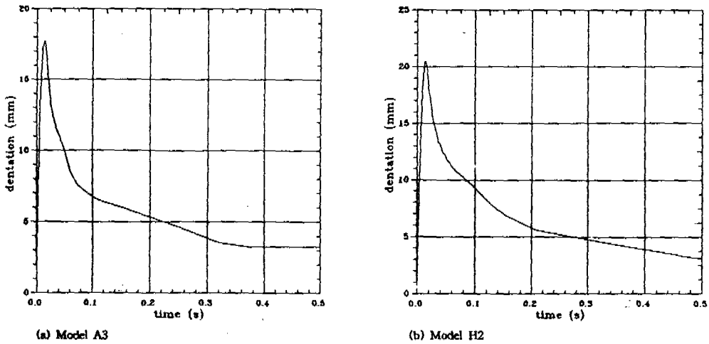
FIGURE 2.3 Time history of depth of dent of Model A3 and H2
