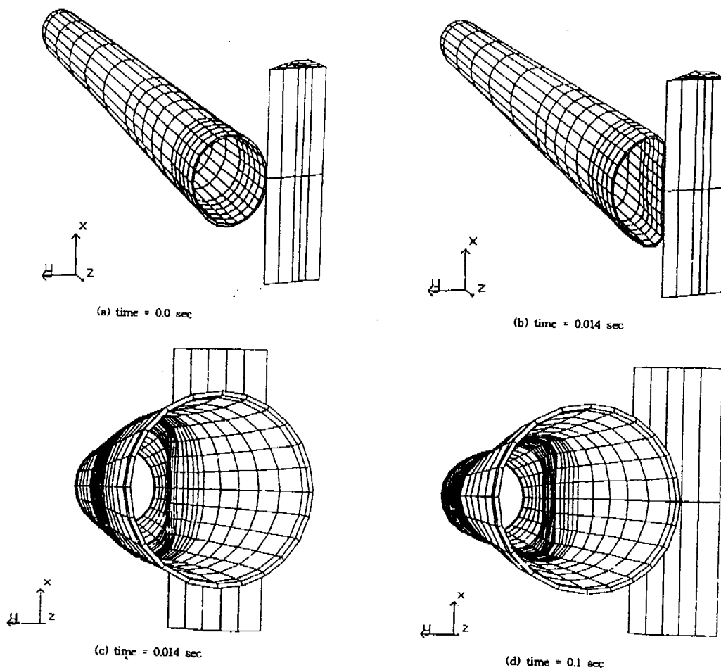
FIGURE 2.1 Numerical meshing and deformed geometry of Model A3
