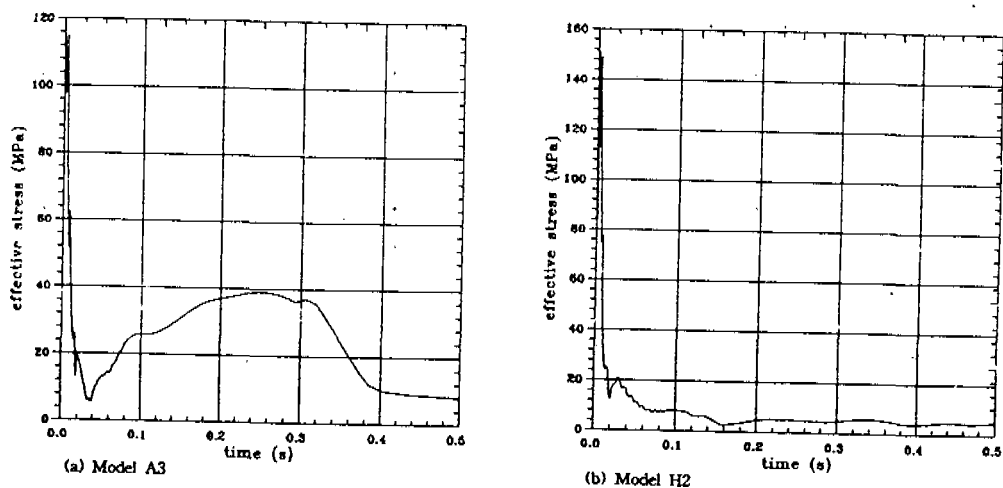
FIGURE 2.2 Time history of effective stress at a point of impact of pipe
