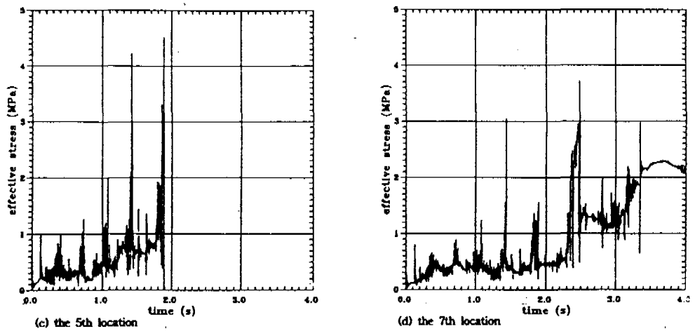
FIGURE 4.5 Time history of effective stress of ices at center
