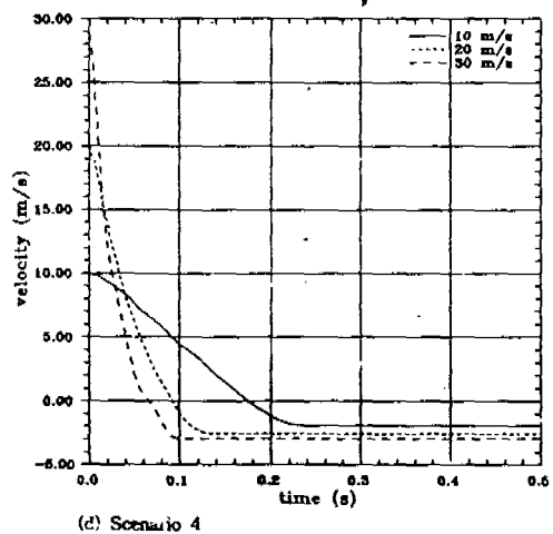
FIGURE 3.4 Time history of velocity of struck pipe
