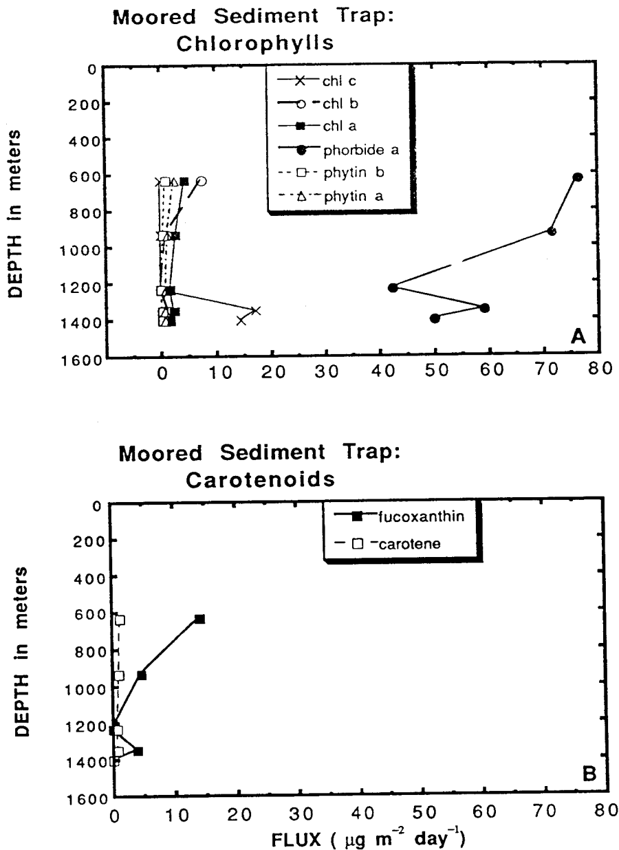
Fig. 8. Vertical profiles of chlorophylls (A) and carotenoids (B) collected by moored sediment traps in the northwest Gulf of Mexico from Nov 1987 to Jan 1988.
