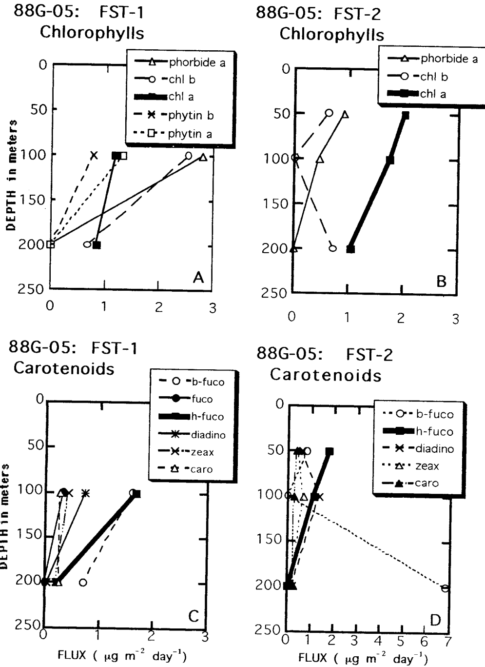
Fig. 7. Fluxes of chlorophylls(A and B) and carotenoids(C and D) intercepted by two deployments of floating sediment traps in a Warm-Core Ring in the northwest Gulf of
