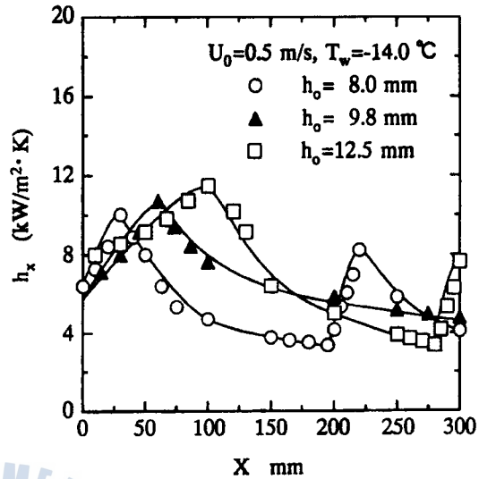
Fig. 7 Local heat transfer characteristics at the lower ice surface
