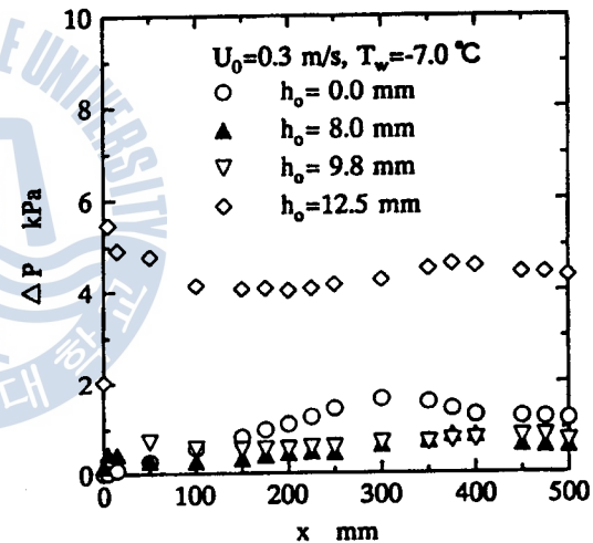
Fig. 9 Pressure-loss characteristics
