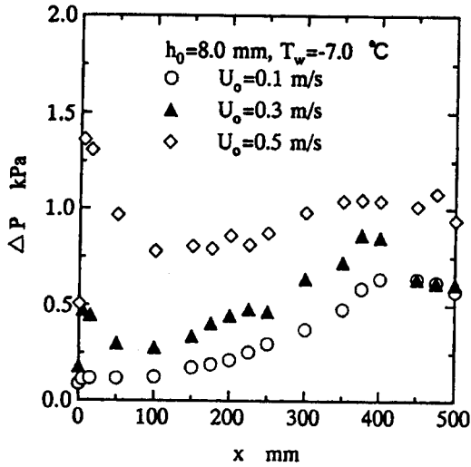
Fig. 10 Pressure-loss characteristics
