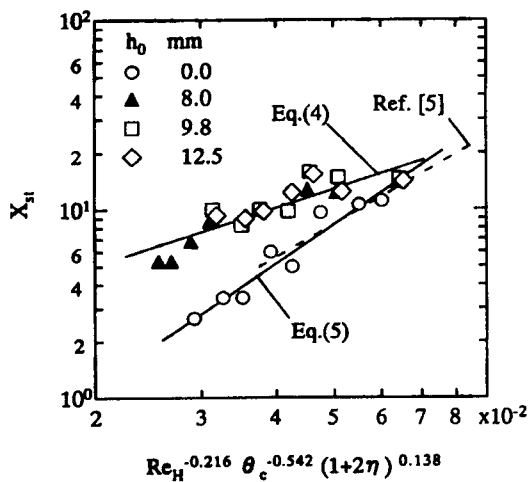
Fig. 6 Correlation of dimensionless icetransition position
