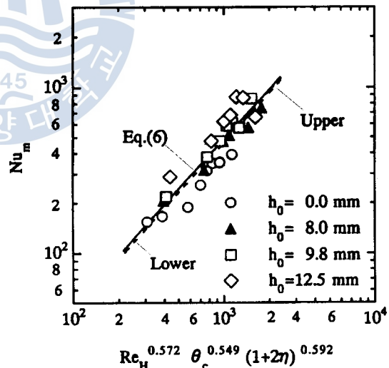
Fig. 8 Correlation of mean Nusselt number
