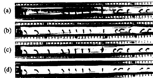
Fig. 2 Effect of orifice height on ice layer profile at steady state for U_0 = 0.5\text{m/s} and T_w = -7.0^\circ\text{C} : (a) h_0 = 0.0\text{mm} , (b) h_0 = 8.0\text{mm} , (c) h_0 = 9.8\text{mm} , (d) h_0 = 12.5\text{mm}
