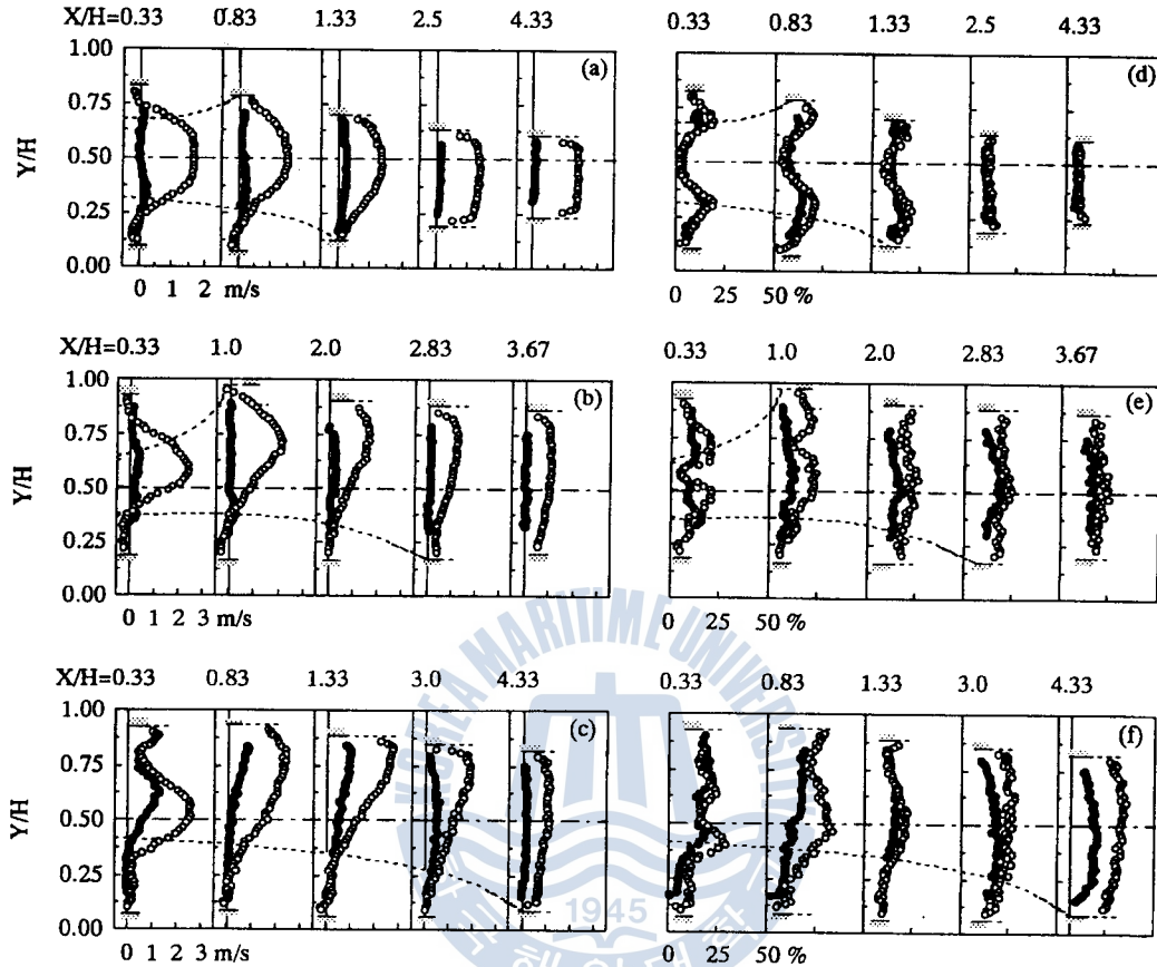
Fig. 3 Effect of orifice height on velocity profile and turbulence intensity at steady state condition for U_0 = 0.5\text{m/s} and T_w = -7.0^\circ\text{C} ; velocity profile( \circ :u, \bullet :v):(a) h_0 = 8.0\text{mm} ,(b) h_0 = 9.8\text{mm} ,(c) h_0 = 12.5\text{mm} ; turbulence intensity( \circ : I_x , \bullet : I_y ):(d) h_0 = 8.0\text{mm} ,(e) h_0 = 9.8\text{mm} ,(f) h_0 = 12.5\text{mm} — ( \circ : Position of the ice surface ---- : Border of stall area)
